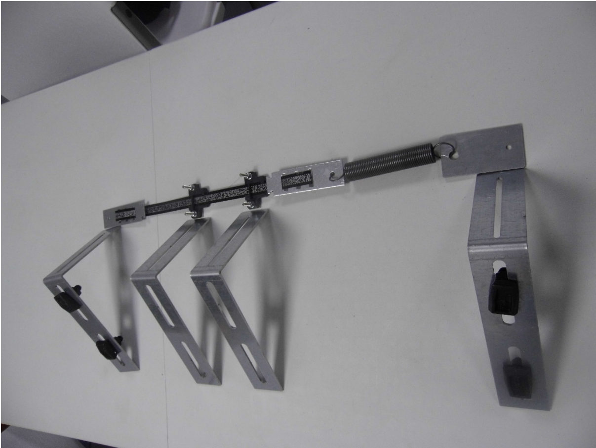
TYPICAL MRL TRACTION CEDES FIXING KIT (BRACKETS TO SUIT NUMBER OF FLOORS)
